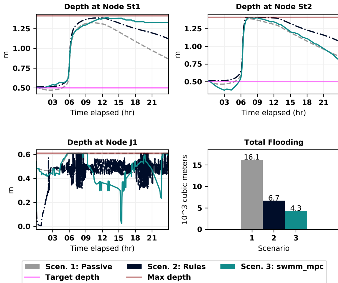
Figure 12: Depth and flooding at system nodes for Case C
